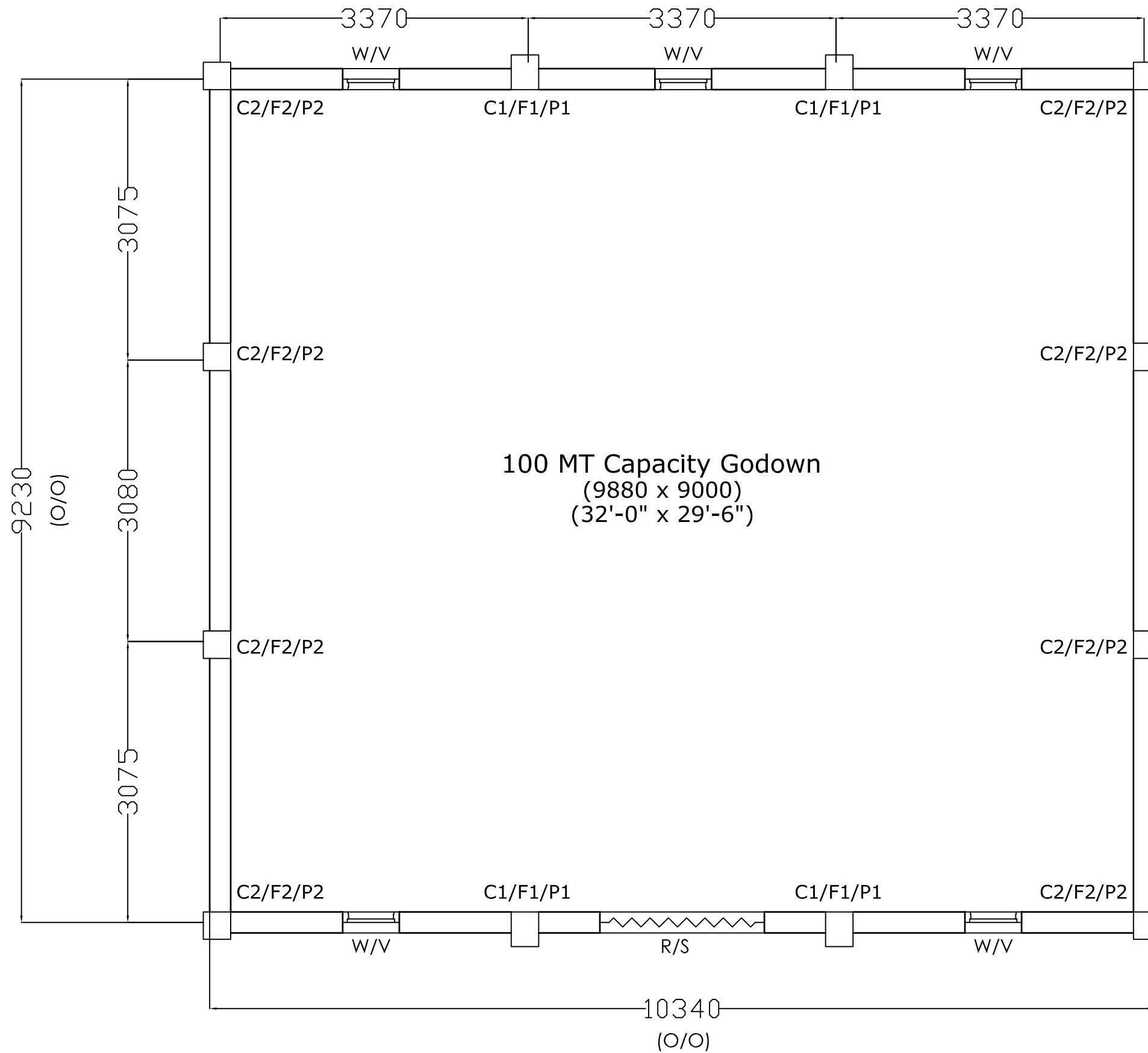
Construction of Godown 100 MT Capacity(Framed Structure)
